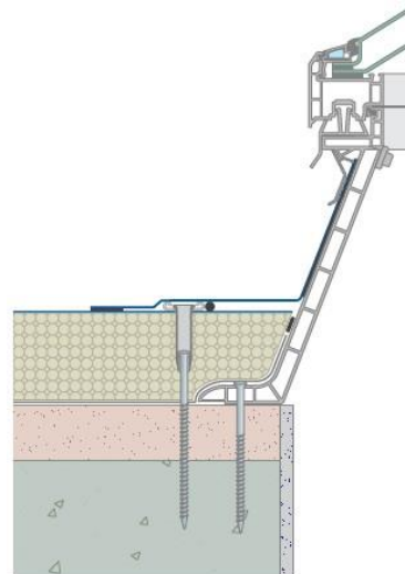
Figure 7: Rooflight Penetration
