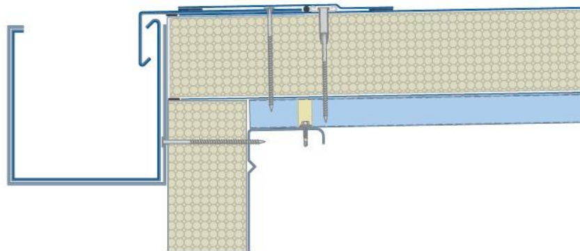
Figure 4: Eaves Gutter
