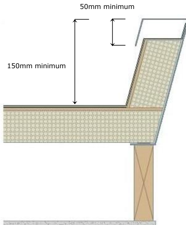
Figure 4: Rooflight penetration
