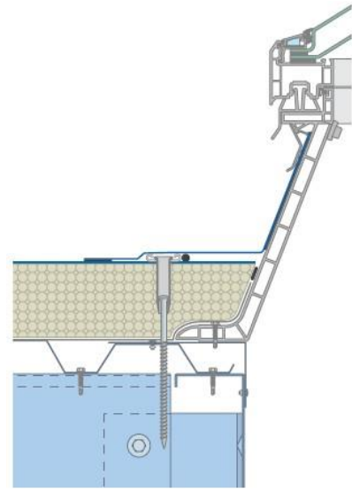
Figure 3: Rooflight Penetration
