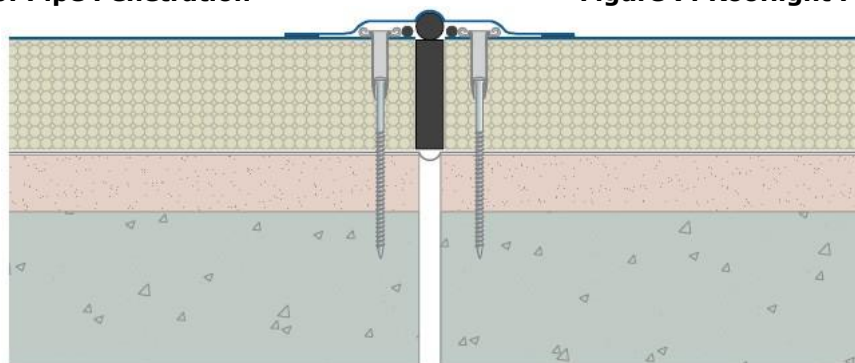
Figure 8: Movement Joint
